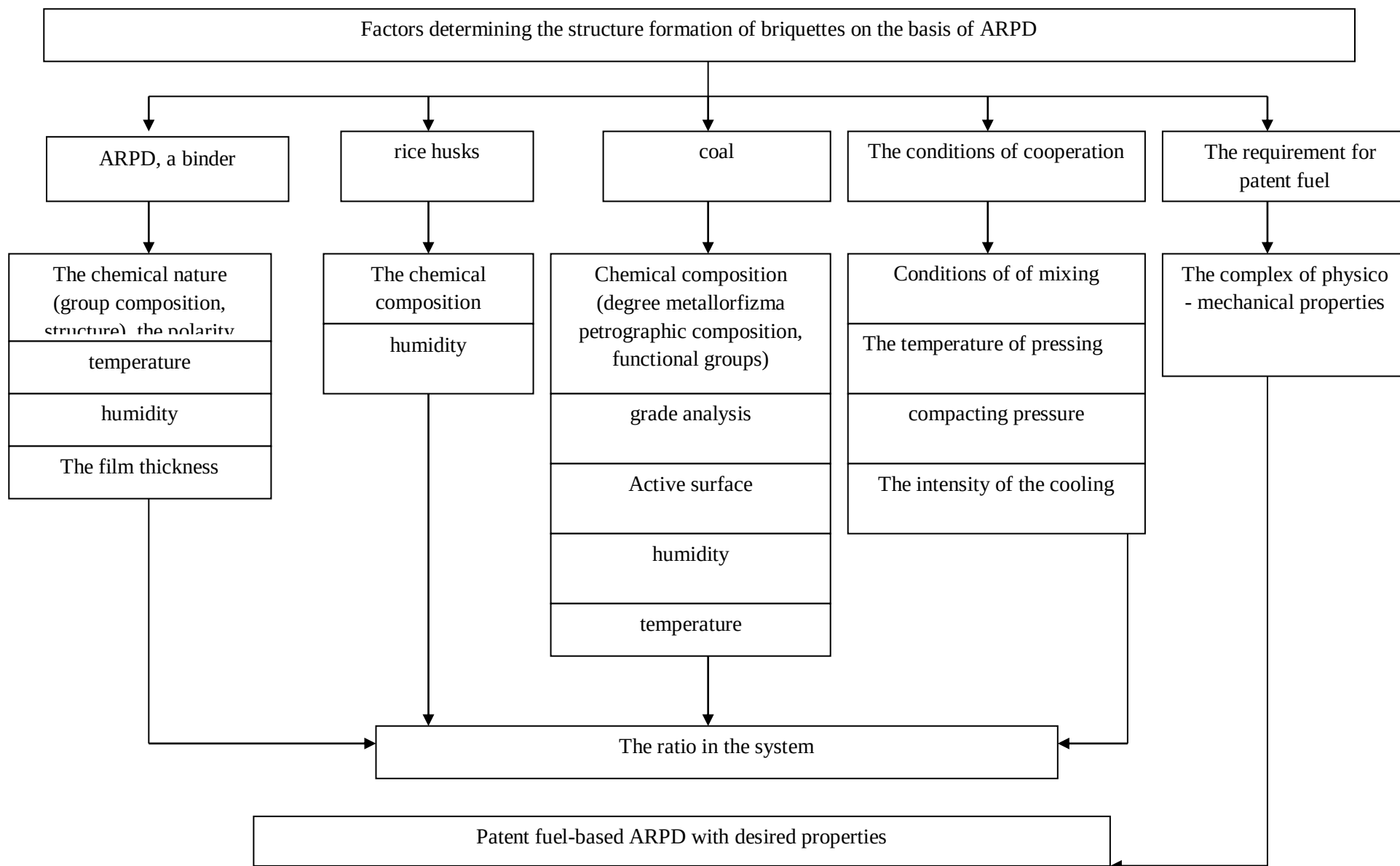
Figure 1 - Analysis of the factors that determine the processes of structure formation of briquetted fuel, based on the ARPD
