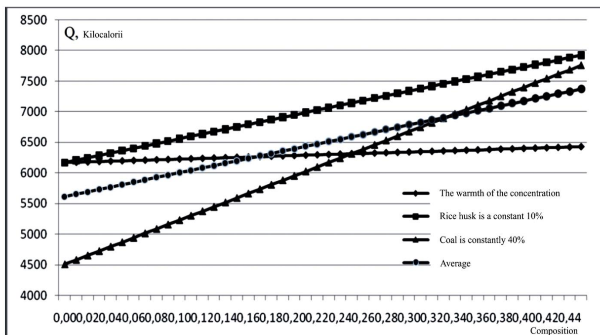
Figure 2 - The value of the heat of combustion of briquettes obtained at different concentrations
